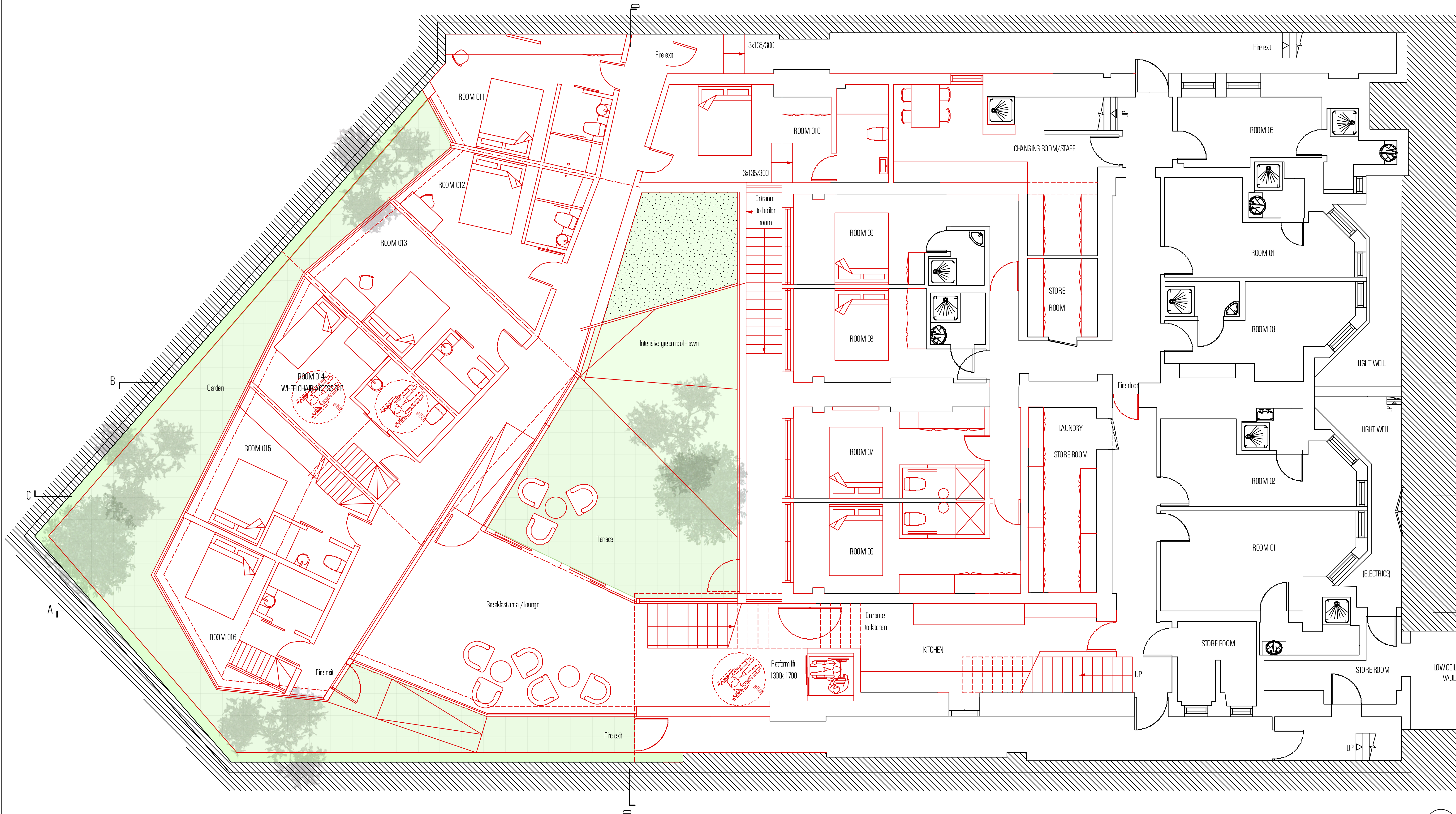
PROPOSED LOWER GROUND FLOOR
