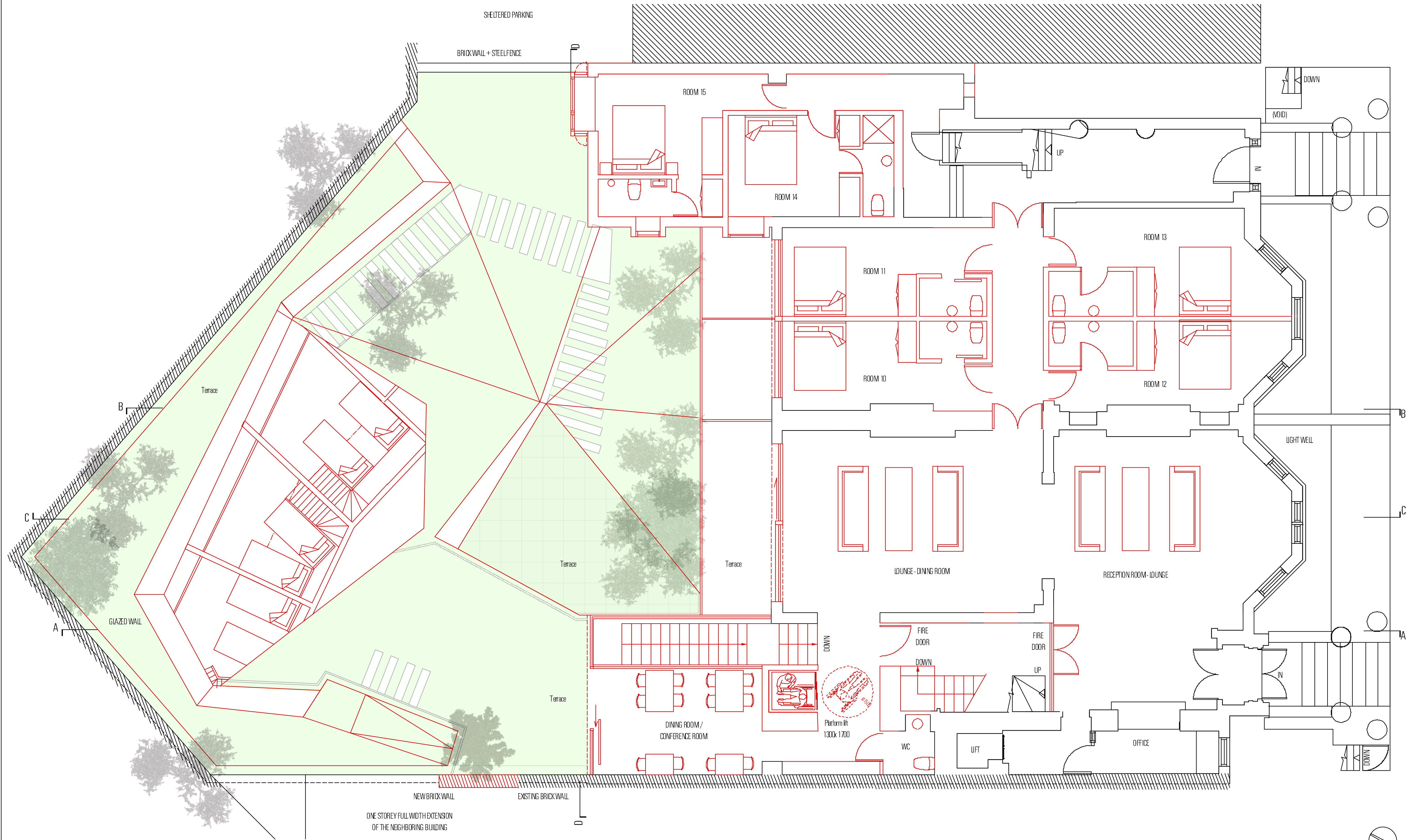
PROPOSED GROUND FLOOR
